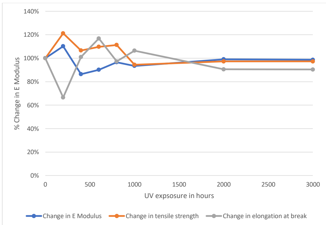
Figure 3 Change in mechanical properties over the course of 3000 hours of UV exposure
